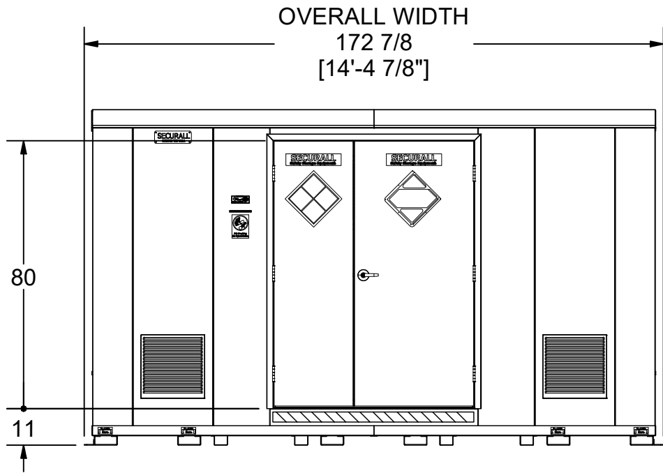
FRONT ELEVATION
